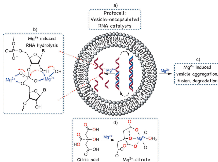
Figure 1. a) A protocell is schematically represented by a set of replicating RNAs that are encapsulated by a lipid vesicle. b) Mg^{2+} ions can catalyze RNA degradation by various mechanisms, including the activation of the phosphate group as well as of the 2'-hydroxy group; the ultimate products of this reaction are a 2',3'-cyclic phosphate and a liberated 5'-hydroxy group, leading to strand cleavage. c) Mg^{2+} ions can also degrade vesicles through their interactions with the carboxylates. d) The structure of citric acid and the core structure of the Mg^{2+} coordination sphere as seen in the crystal structure of magnesium citrate; in this highly networked structure, all carboxylates are interacting with the Mg^{2+} ion, leaving one potentially labile coordinating water molecule (Ref. [11]).
